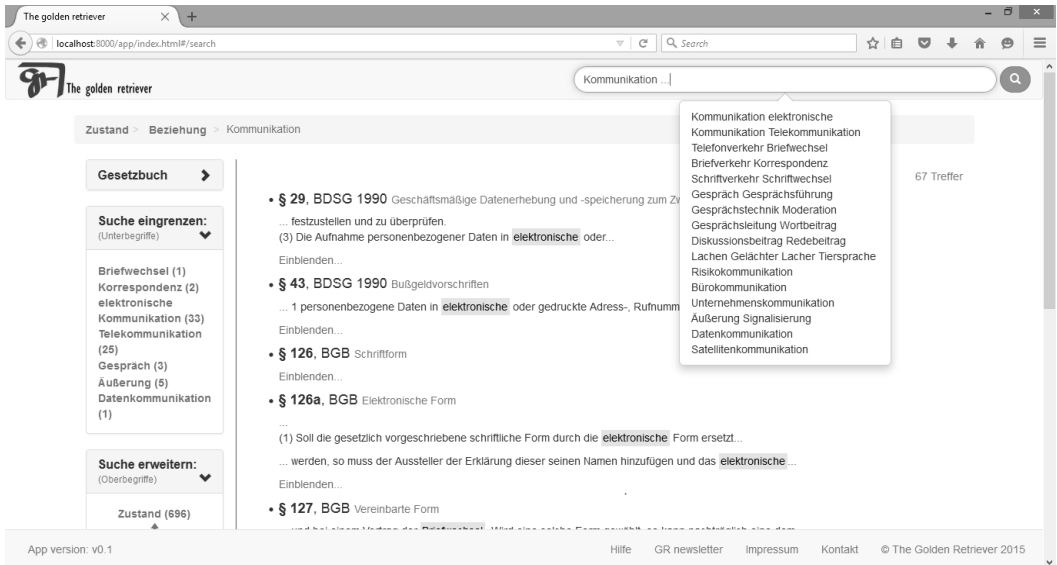
Figure 5.2: System features
