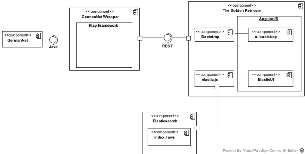
Figure 5.1 Overall reference architecture of the system fostering easy adaptability and reuse of components.
