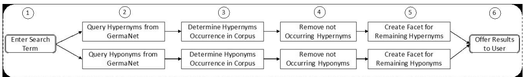
Figure 4.4 Search Query Reformulation Process
